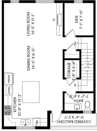
Main Floor - 688 sq.ft. Ceiling height - 9' 0"
