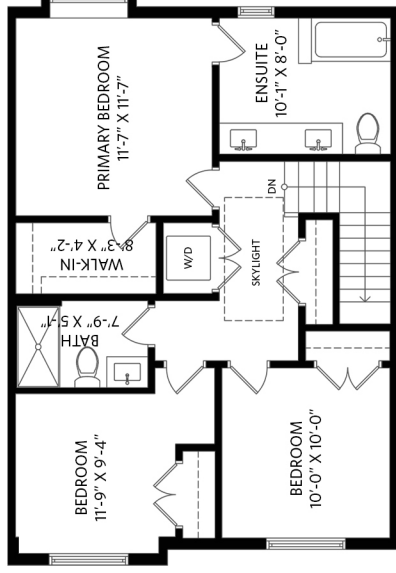
Upper Floor - 747 sq.ft. Ceiling height - 8' 3"
