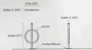
Model: Maglin MBR100 Series Materials: All steel components with powdercoat finish * minimum spacing = 1.0m between racks
