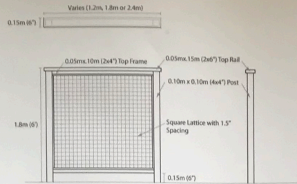
WOOD AND LATTICE PRIVACY SCREEN SCALE = 1:25 (1/2" = 1'-0")
