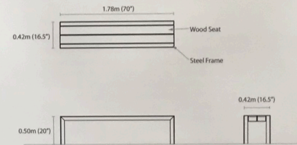
Model: Maglin MB1050B Series Bench (backless) Materials: Formed Steel Frame with Wood Seat
